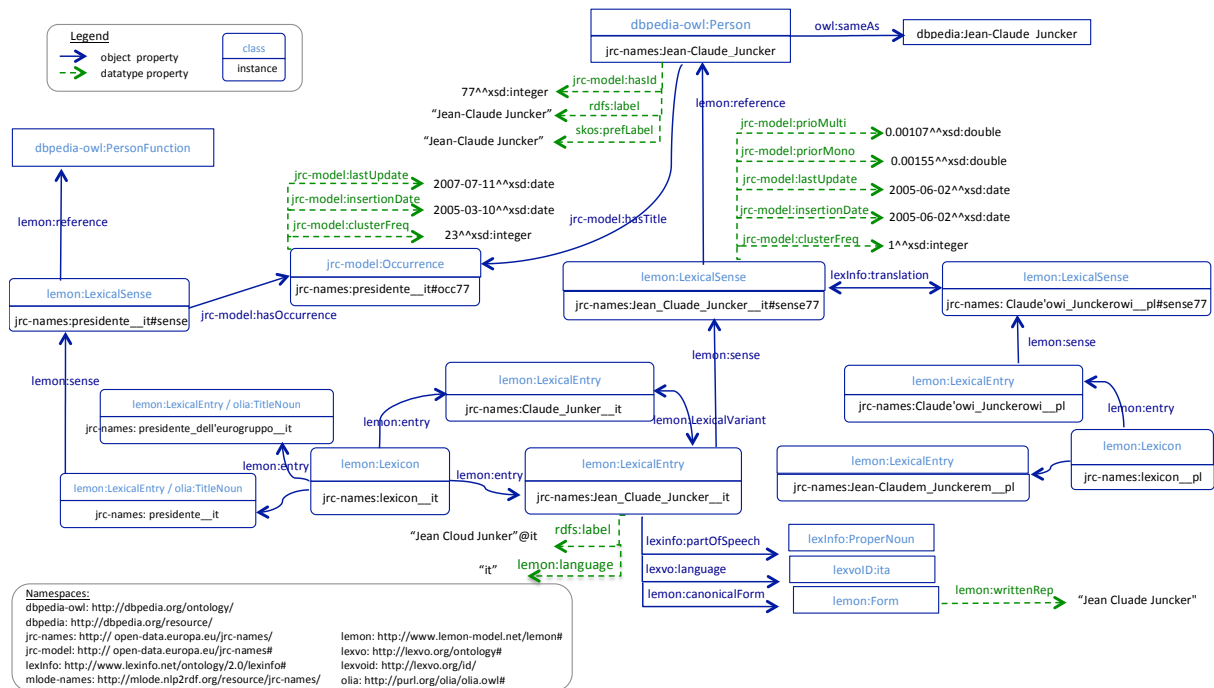
Figure 2. Graphical illustration of JRC-Names data representation, with the example of the entity Jean-Claude Juncker .
