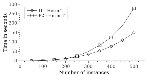
Fig. 12. Average reasoning time as a function of the number of instances
