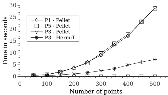
Fig. 11. Average reasoning time as a function of the number of points
