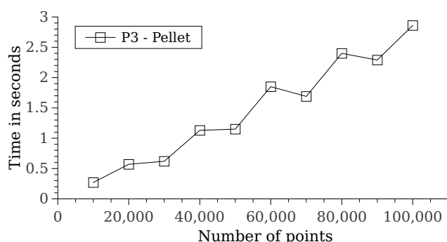
Fig. 14. Average reasoning time as a function of the number of points
