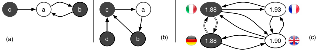
Fig. 2. Example of (a) an AF , (b) a bipolar AF , and (c) example provided in the introduction modeled as a bipolar AF , where single lines represent attacks and double lines represent support.
