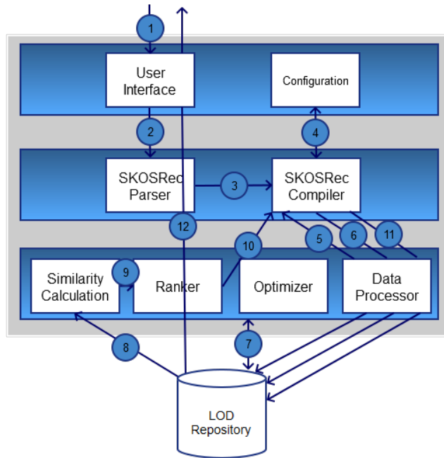
Fig. 1. Architecture and workflow of the SKOSRec engine
