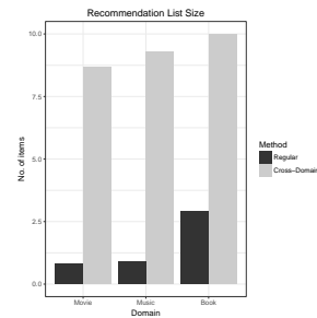
Fig. 10. Mean recommendation list sizes for SPARQL and SKOS-Rec cross-domain requests (TC4)
