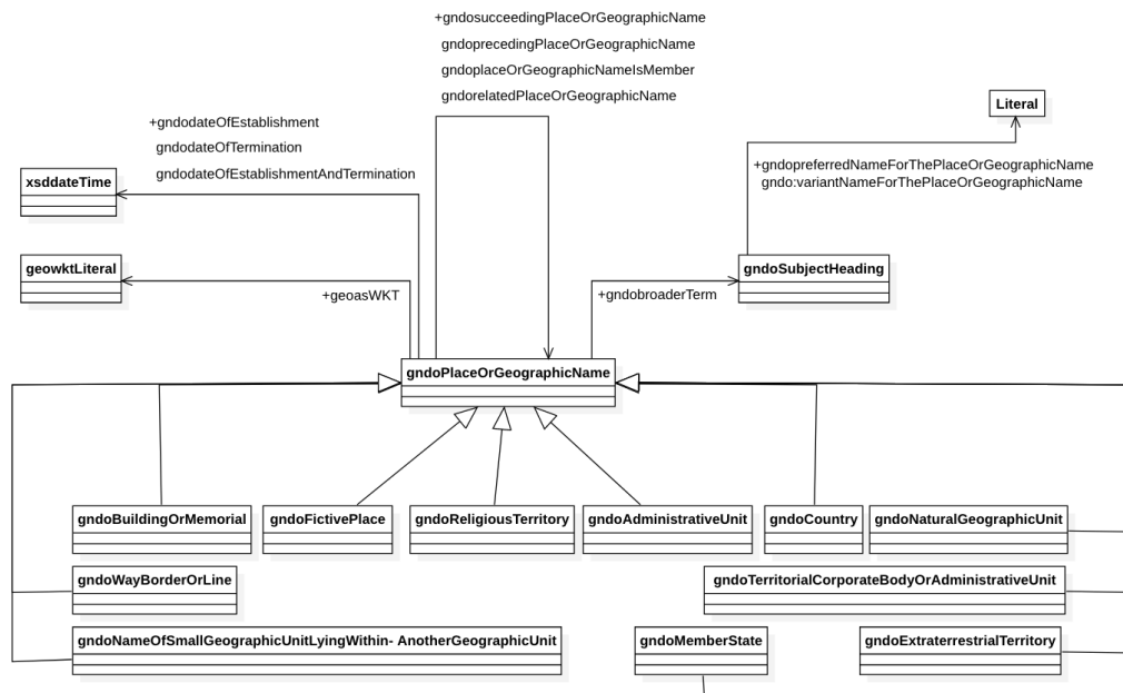
Fig. 2. UML representation of the GND classes discussed in Section 4.2
