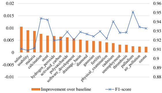
Fig. 6. F1 improvements over the cold baseline for individual FoS datasets trained using LR, with F1 in the second axis.
