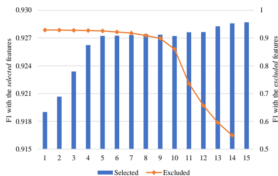
Fig. 2. Changes in the F1 of the classification results using mutual_info_classif as the scoring function with f=[1, \dots, 15] in the x-axis, with the results of classifications using the excluded features shown in the second y-axis.
