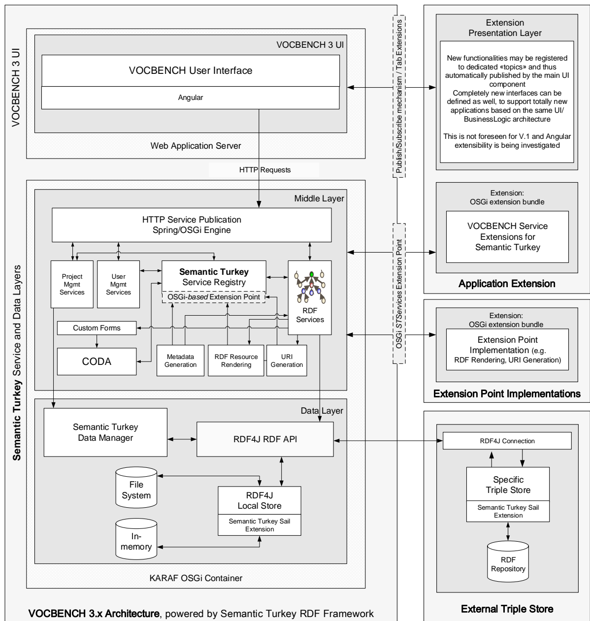
Figure 1. VocBench 3 Architecture
