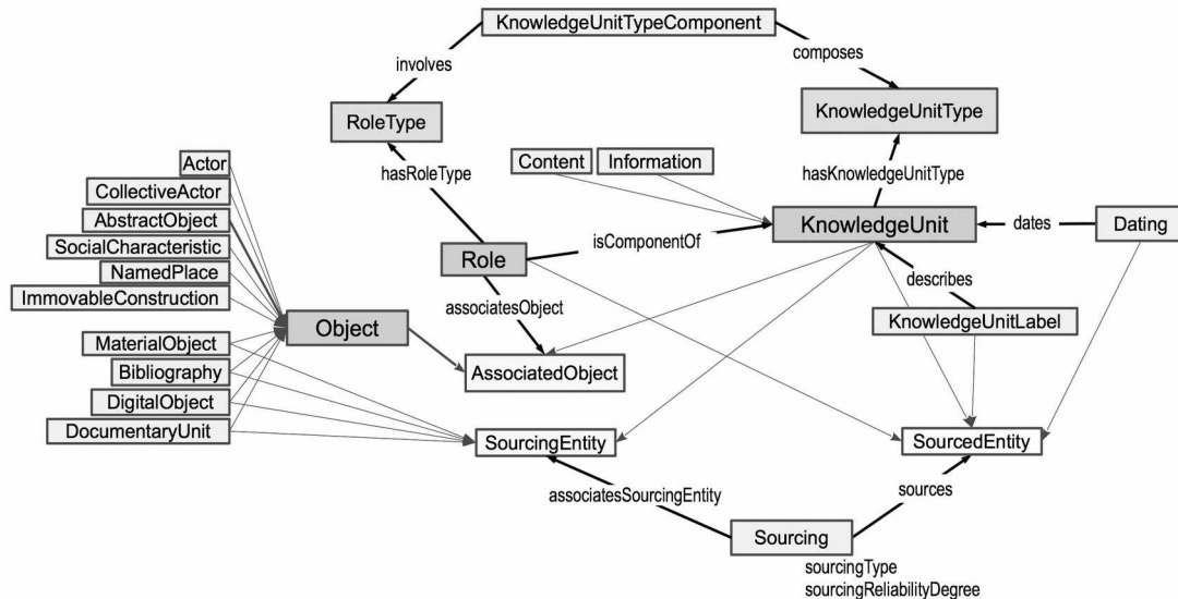
Fig. 1. Ontology of the symogih.org project -version 0.2.1
