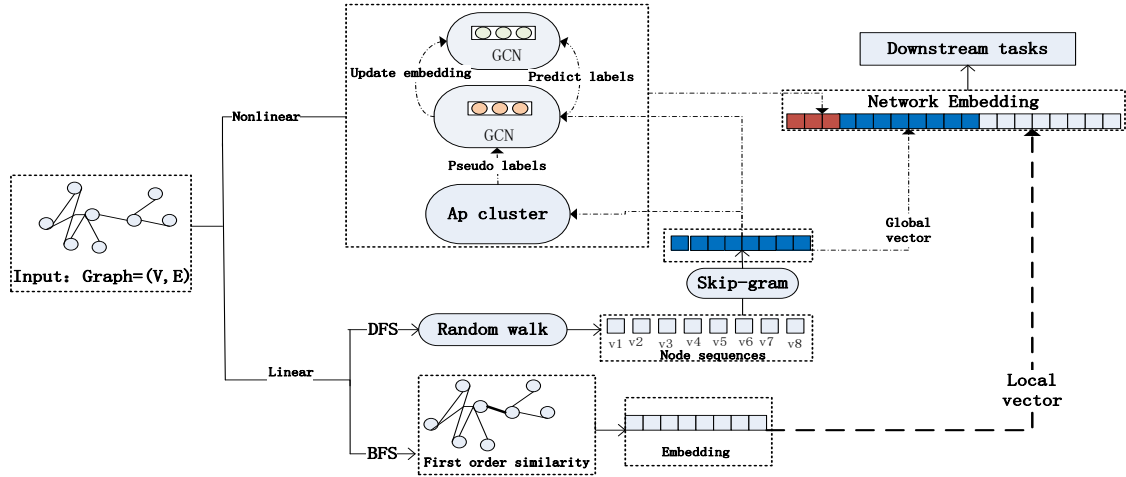
Fig.2. Model architecture.
