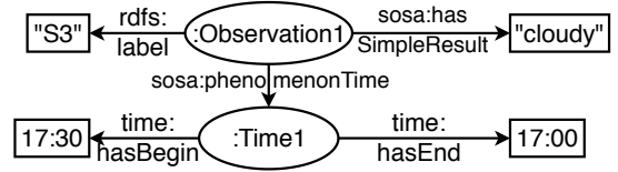
Fig. 5. Incorrect mapping of the third line in Fig. 1 to the ontology in Fig. 2. For brevity, we omit rdf:type relations.
