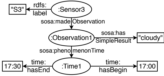
Fig. 4. Correct mapping of the third line in Fig. 1 to the ontology in Fig. 2. For brevity, we omit rdf:type relations.
