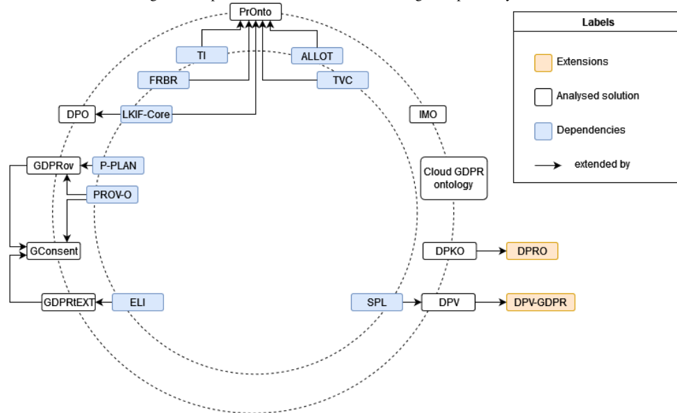
Fig. 3. Data protection vocabularies and ontologies dependency chart.
