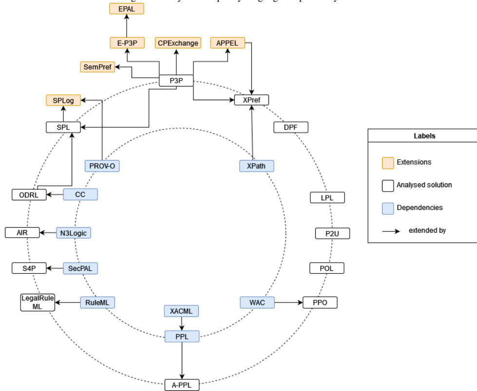
Fig. 2. Privacy-related policy languages dependency chart.
