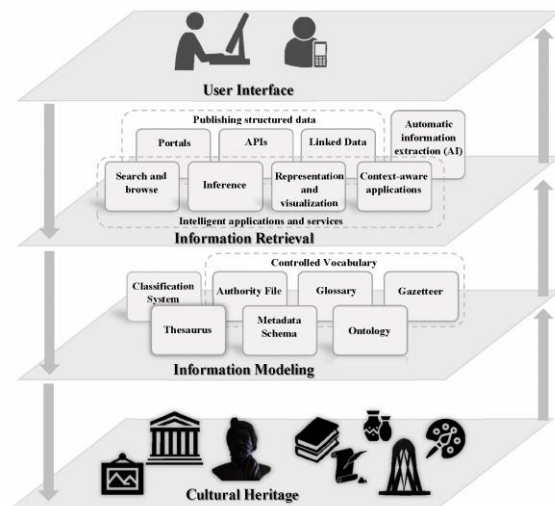
Fig. 1. Conceptual framework of the research.
