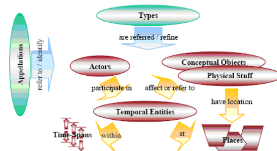
Fig. 3. Major concepts of the event-centric CIDOC CRM model [39].
