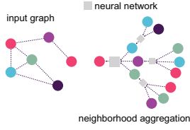
Graph Neural Network (GNN)
