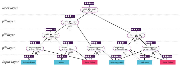
Recursive Neural Knowledge Networks (RNKN)
