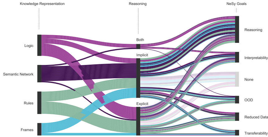
Fig. 23. Knowledge Representation, Type of Reasoning, and Goals. What is noteworthy, is that when Semantic Networks are utilized, reasoning is almost always done implicitly. The two exception are [83], and [77]. However, [83] utilizes FOL for explicit reasoning rather than its network component. On the other hand, [77] generate a novel interpretable reasoning graph as the output of their model.
