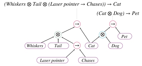
Fig. 26. Neuro-symbolic architectures represented in Table 4
