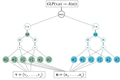
Logic Tensor Networks (LTN)
