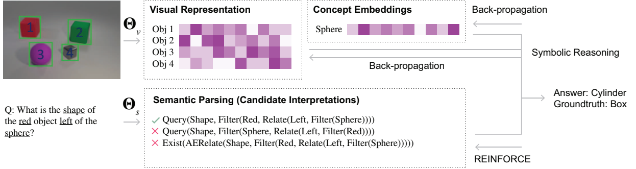
Fig. 31. Type 3 Cooperative . The Neuro-Symbolic Concept Learner (NS-CL) jointly learns visual concepts, words, and semantic parsing of sentences without any explicit annotations. Given an input image, the visual perception module detects objects in the scene and extracts a deep, latent representation for each of them. The semantic parsing module translates an input question in natural language into an executable program given a domain specific language (DSL). The generated programs have a hierarchical structure of symbolic, functional modules, each fulfilling a specific operation over the scene representation. The explicit program semantics enjoys compositionality, interpretability, and generalizability [137].
