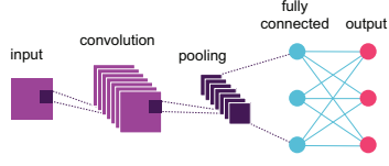
Convolutional Neural Network (CNN)
