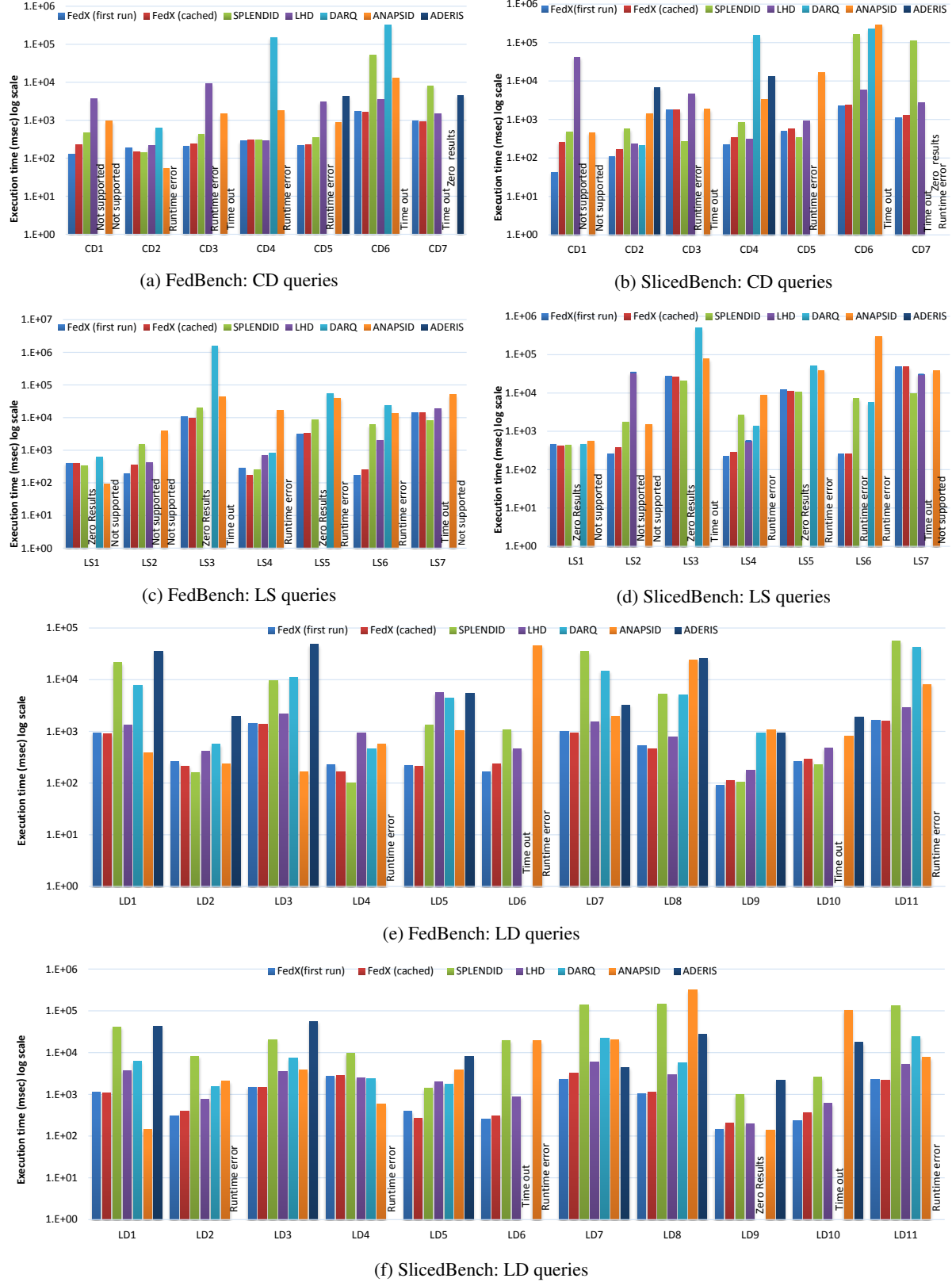
Fig. 7. Comparison of pure query execution time (without source selection time) for FedBench and SlicedBench
